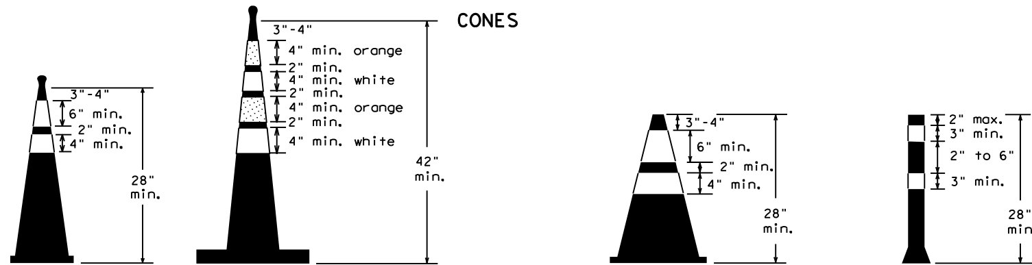
Two-Piece cones
