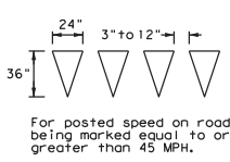
YIELD LINES
