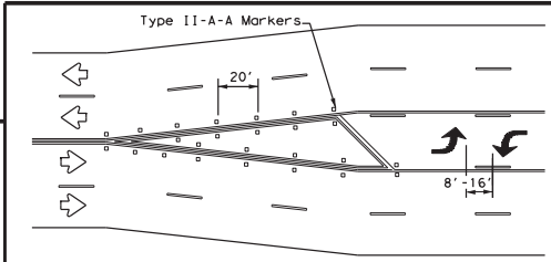
TYPICAL TRANSITION FOR TWLTL AND DIVIDED HIGHWAY
