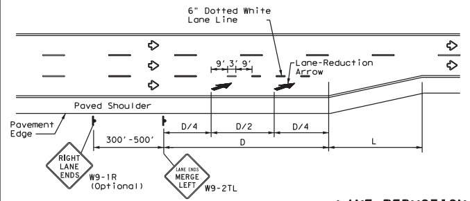
LANE REDUCTION
