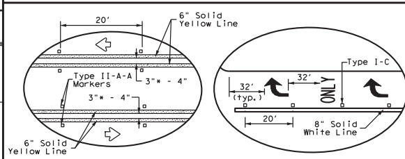
DETAIL A
