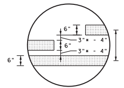
TYPICAL MULTI-LANE, TWO-WAY PAVEMENT MARKINGS THROUGH INTERSECTIONS
