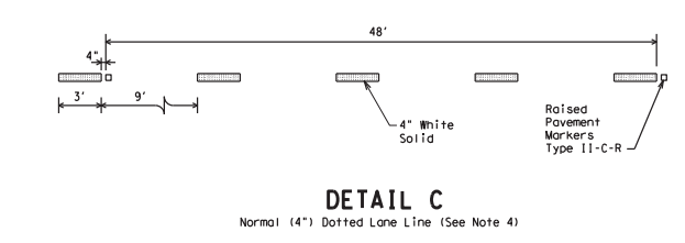
PARALLEL DECELERATION LANE
