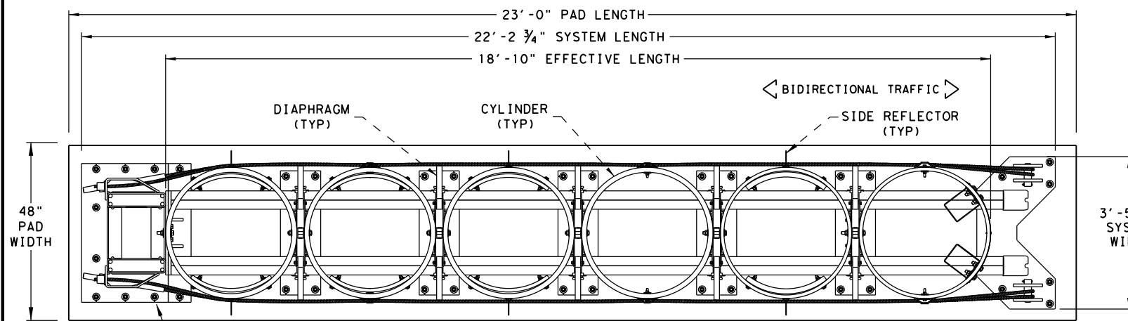
PLAN VIEW
