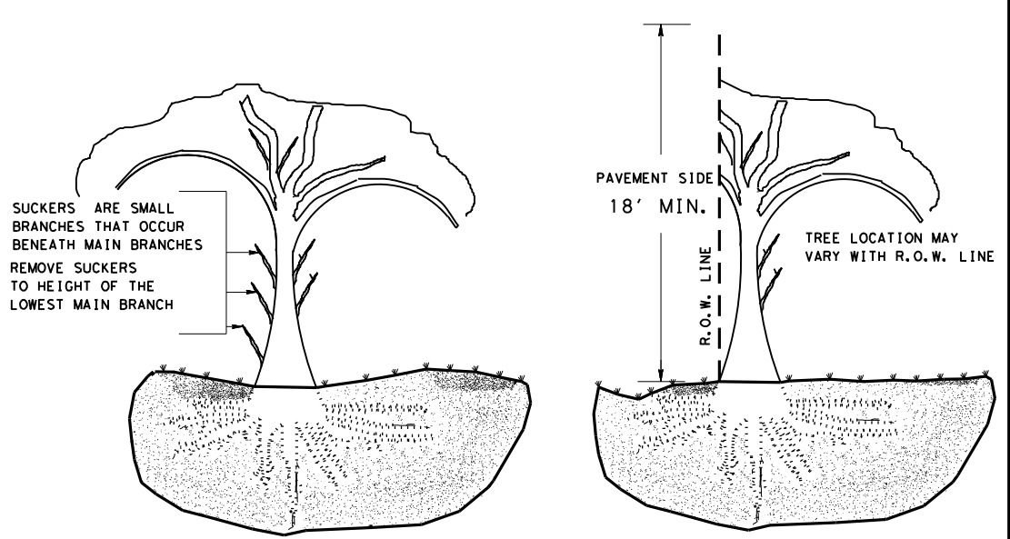
REMOVE ALL LIMBS ON PAVEMENT SIDE TO 18' ABOVE SURROUNDING NATURAL GROUND WHEN TREE IS AT R.O.W.
