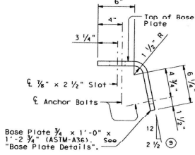
SECTION A-A OF 9" HIGH CURBS (Showing example of 8" Min width curb, wider curbs similar)
