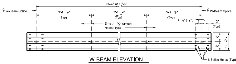
W-BEAM ELEVATION
