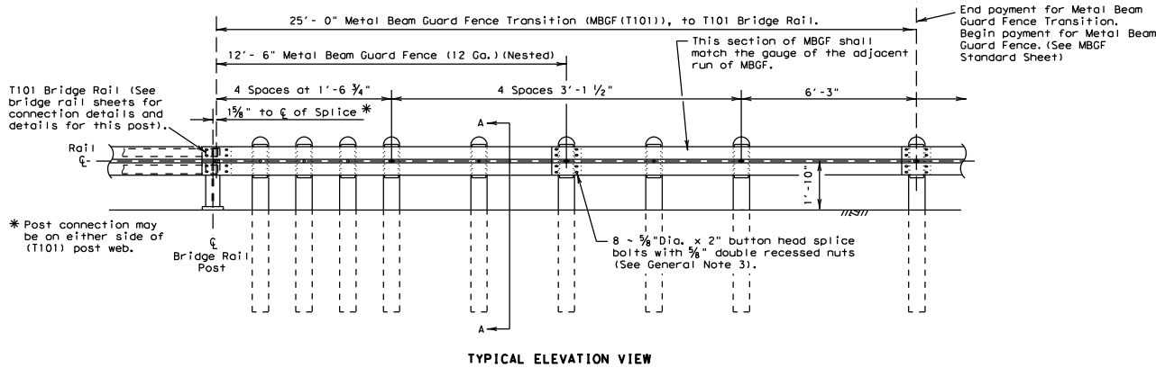
TYPICAL ELEVATION VIEW
