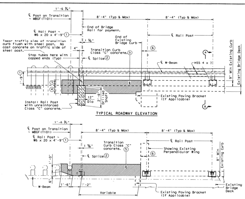
EXAMPLE "B" RETROFIT WITH PERPENDICULAR WING (Showing 9' high and 8" wide curbs, higher and wider curbs similar)
