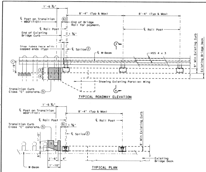
EXAMPLE "A" RETROFIT WITH PARALLEL WING (Showing 9' high and 8" wide curbs, higher and wider curbs similar)
