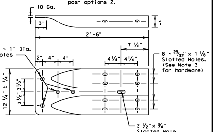
TERMINAL CONNECTOR
