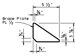
BRACE PLATE DETAILS
