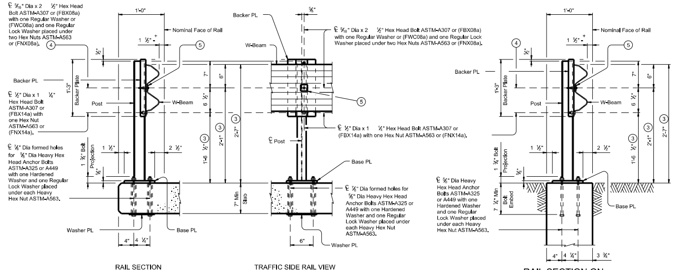
RAIL SECTION RAIL DETAILS ON BRIDGE SLAB
