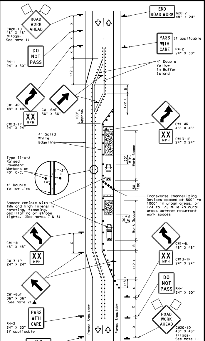
TCP (2-3b) 2-LANE ROADWAY WITH PAVED SHOULDERS ONE LANE CLOSED INADEQUATE FIELD OF VIEW
