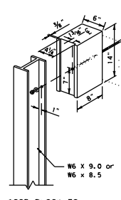
WOOD BLOCK TO STEEL POST
