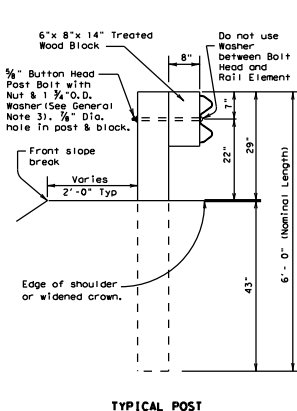
TYPICAL POST
