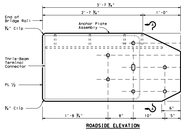
ROADSIDE ELEVATION
