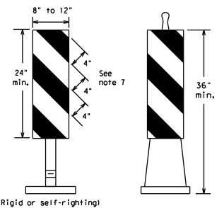
PORTABLE (Rigid or self-righting)
