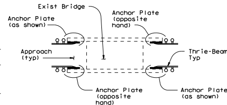
LOCATION DETAILS
