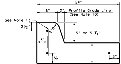
TYPE II CURB AND GUTTER 5" - 5 3/4" HEIGHT
