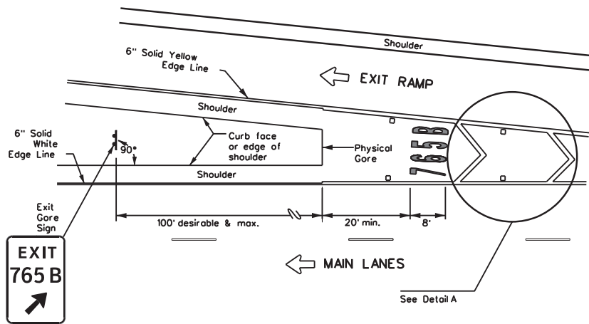
MARKINGS WITH EXIT NUMBER
