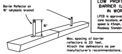
LOW PROFILE CONCRETE BARRIER (LPCB)
