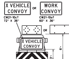
TRAIL/SHADOW VEHICLE B
