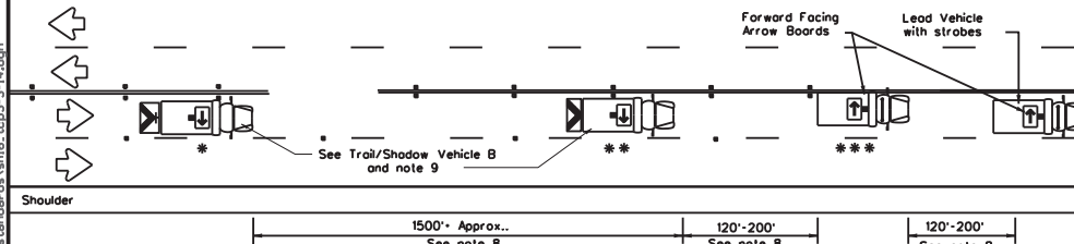
TCP (3-3d) UNDIVIDED MULTILANE HIGHWAY
