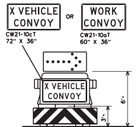
TRAIL/SHADOW VEHICLE A
