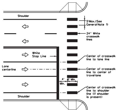
HIGH-VISIBILITY LONGITUDINAL CROSSWALK AT CONTROLLED APPROACH
