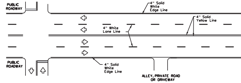
TYPICAL MULTI-LANE, TWO-WAY PAVEMENT MARKINGS THROUGH INTERSECTIONS
