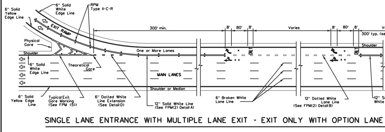
MULTIPLE LANE EXIT ONLY
