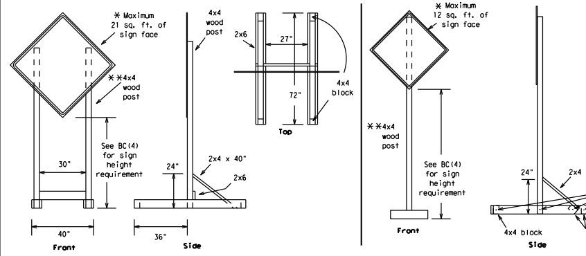
SKID MOUNTED WOOD SIGN SUPPORTS * LONG/INTERMEDIATE TERM STATIONARY - PORTABLE SKID MOUNTED SIGN SUPPORTS
