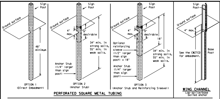
GROUND MOUNTED SQUARE METAL TUBING SIGN SUPPORTS Refer to the CWZTCO and the manufacturer's installation procedure for each type sign support. The maximum sign square footage shall adhere to the manufacturer's recommendation. Two post installations can be used for larger signs.
