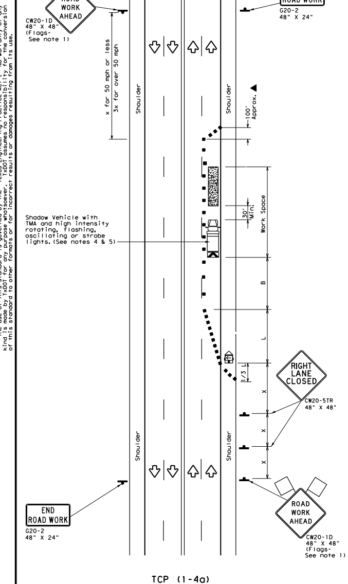
TCP (1-4a) ONE LANE CLOSED
