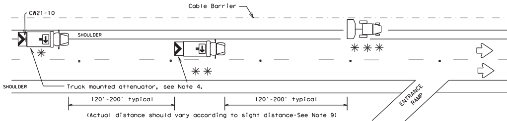
Divided Multilane Highway with Cable Barrier
