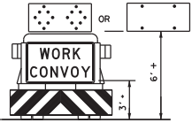
TYPICAL TRAIL VEHICLE
