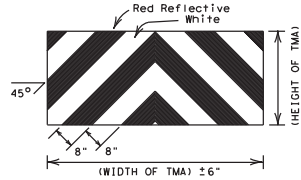
STRIPING FOR TMA
